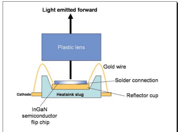
Fig. 5. Diagram of recent high-power LEDs.
