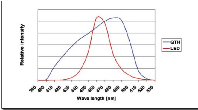
Fig. 3. Characteristic spectra of QTH and LED lamps.
