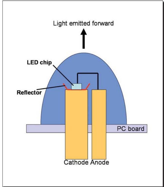
Fig. 4. Diagram of old-styled conventional LED lamps.
